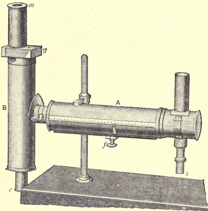
FIG. 10.—Weber Photometer.
